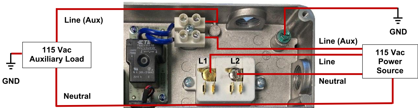
Auxiliary Load Relay Wiring, 115 Vac Power
