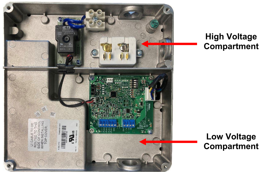
High and Low Voltage Compartments
